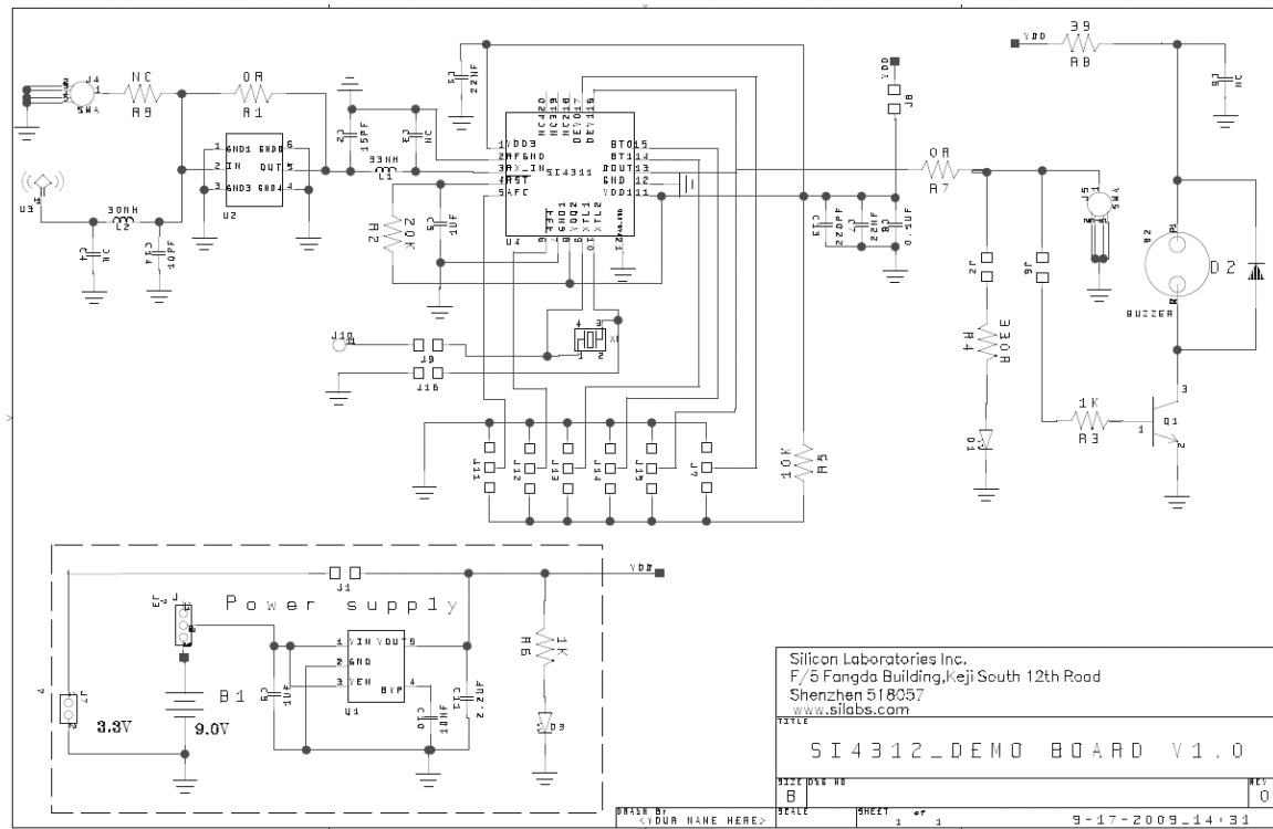
Figure 3. Si4312-DEMO Schematic
